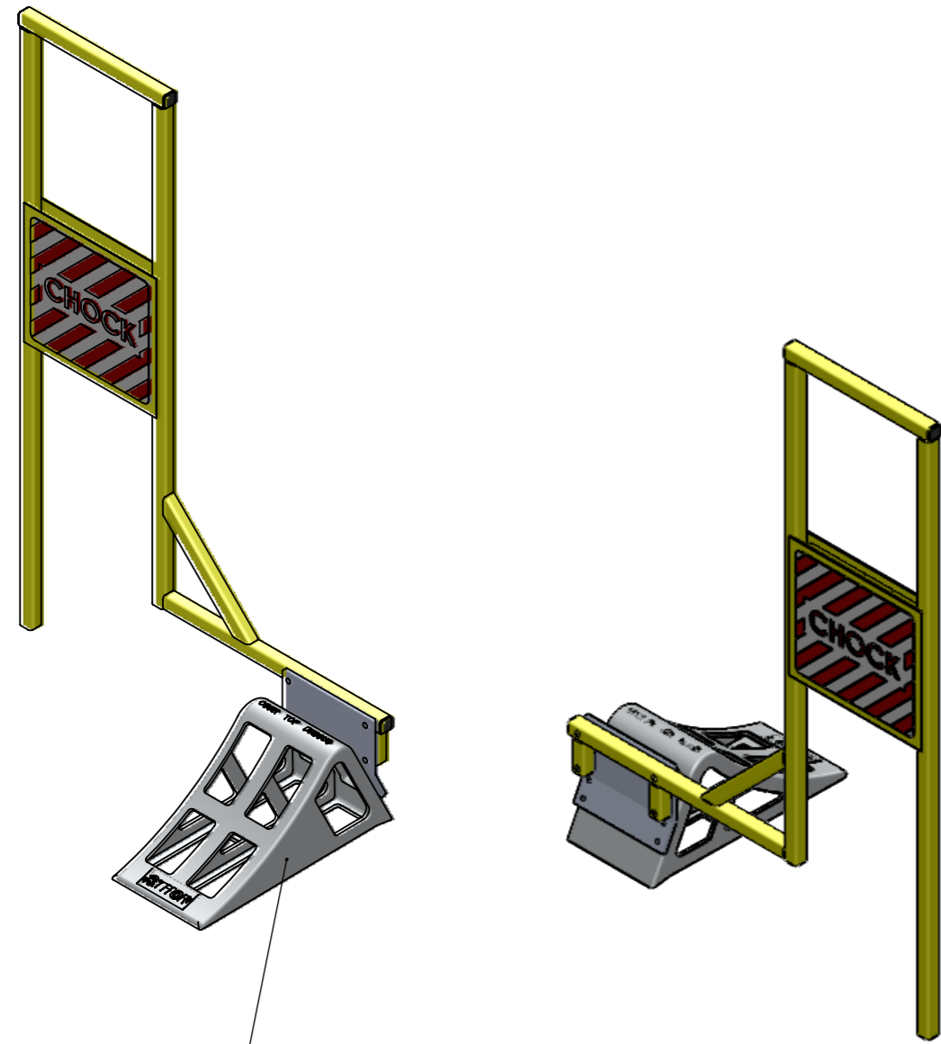
TWC-3 Aluminium wheel chock
