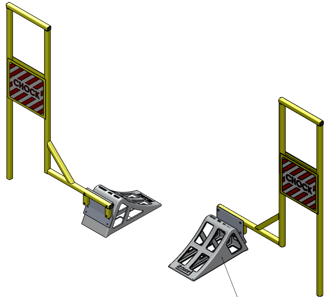
TWC-3 Aluminium wheel chock
